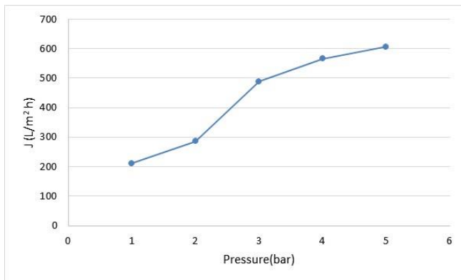
Figure 2. Average distilled water flow for PES 10 kDa membrane
