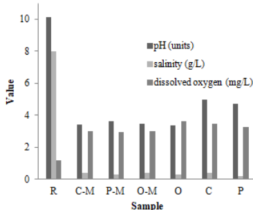
Figure 3. Waste water pH, salinity and dissolved oxygen for all variants of natural dyeings
