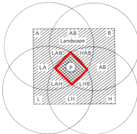
Figure 2. Diagram of the possible intractions between the Litosphere (L), the Hydrosphere (H), the Atmosphere (A) and Biosphere (B). Whenthey interact they form the Pedosphere (P). (modified after Mattson, 1938)
