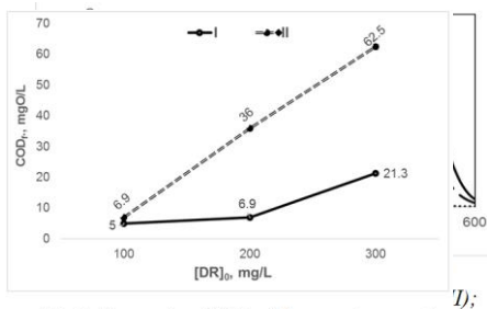
Fig.2. Remaning COD of first and second systems after coagulation; [Al 3+ ] = 4.32 mg/L respectively
