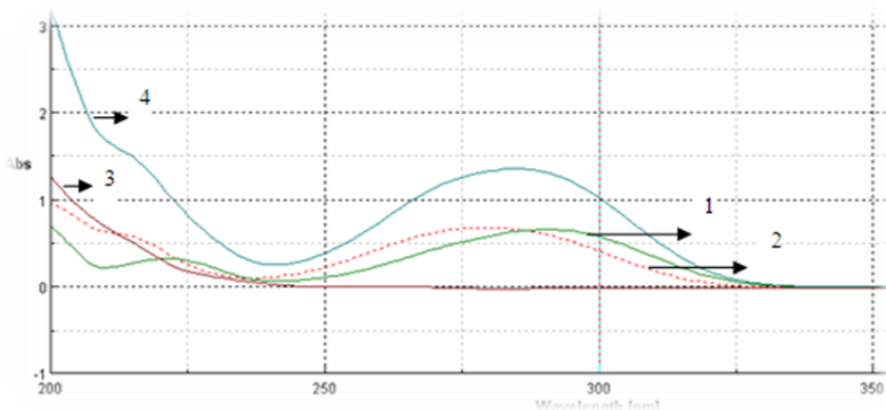
Figure 2. Absorption spectra of: 1. PH·HCl (11.04 \mu\text{g}/\text{mL} ), 2. PHA·HCl (10.72 \mu\text{g}/\text{mL} ), 3. Lid (9.28 \mu\text{g}/\text{mL} ) and 4. mixture of PH·HCl, PHA·HCl and Lid (11.04 - 10.72 - 9.28 \mu\text{g}/\text{mL} )
